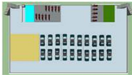
GAMBAR 2. DENAH AREA BASEMENT BALAI PERTIWI
