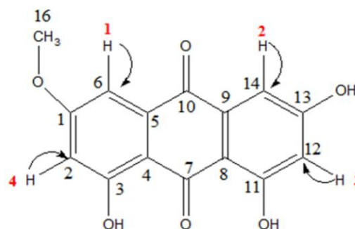
Figure 2. Structure of Isolate 1.1, (HMQC =
