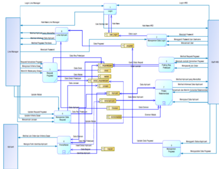
Gambar 2. Data Flow Diagram Lv 1.
