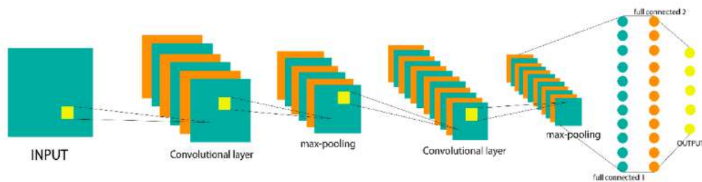
FIGURE 2: LeNet architecture
