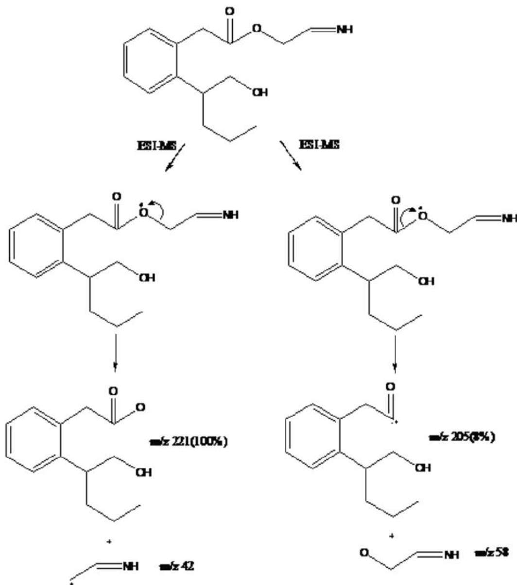
Figure 6: Estimation fragmentation pattern of isolate 2
