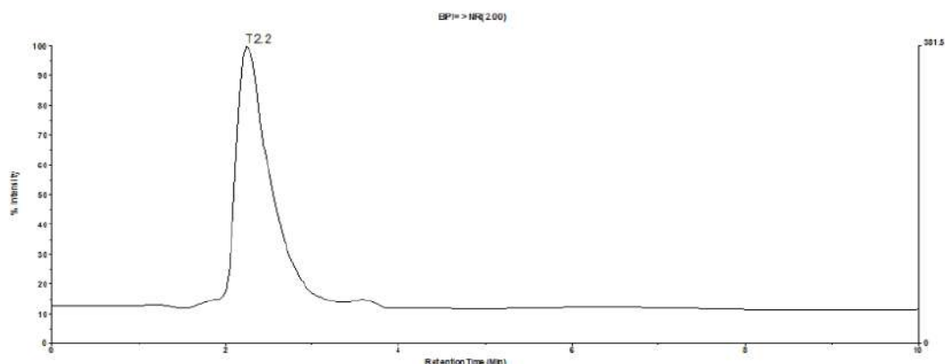
Figure 2: Fraction 2 Chromatogram
