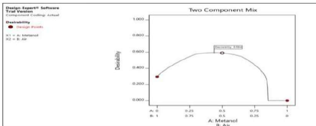
Figure 5: Response Desirability of Metanol-Water Solvent Combination
