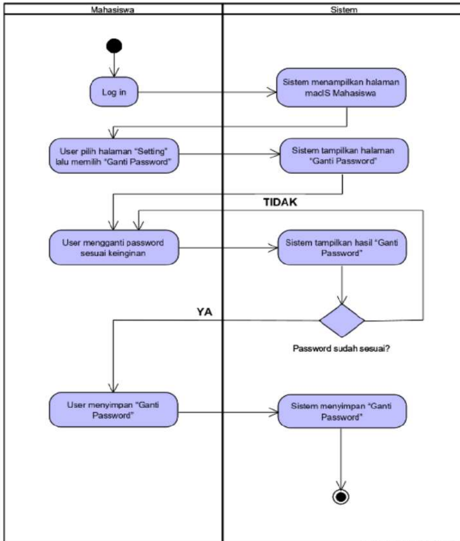
Gambar 8 Diagram Aktivitas Setting – Ganti Password
