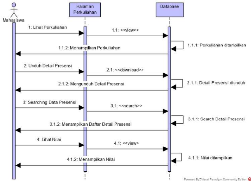
Gambar 11 Sequence Diagram Perkuliahan
