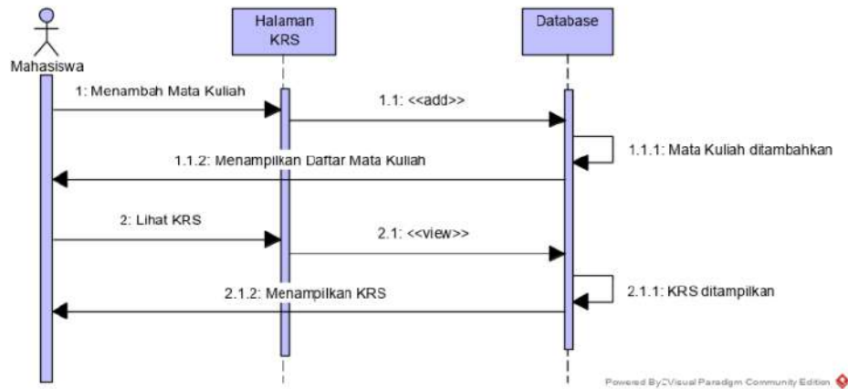
Gambar 10 Sequence Diagram KRS
