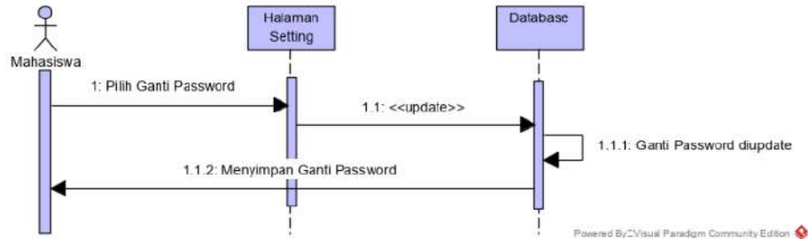
Gambar 12 Sequence Diagram Setting
