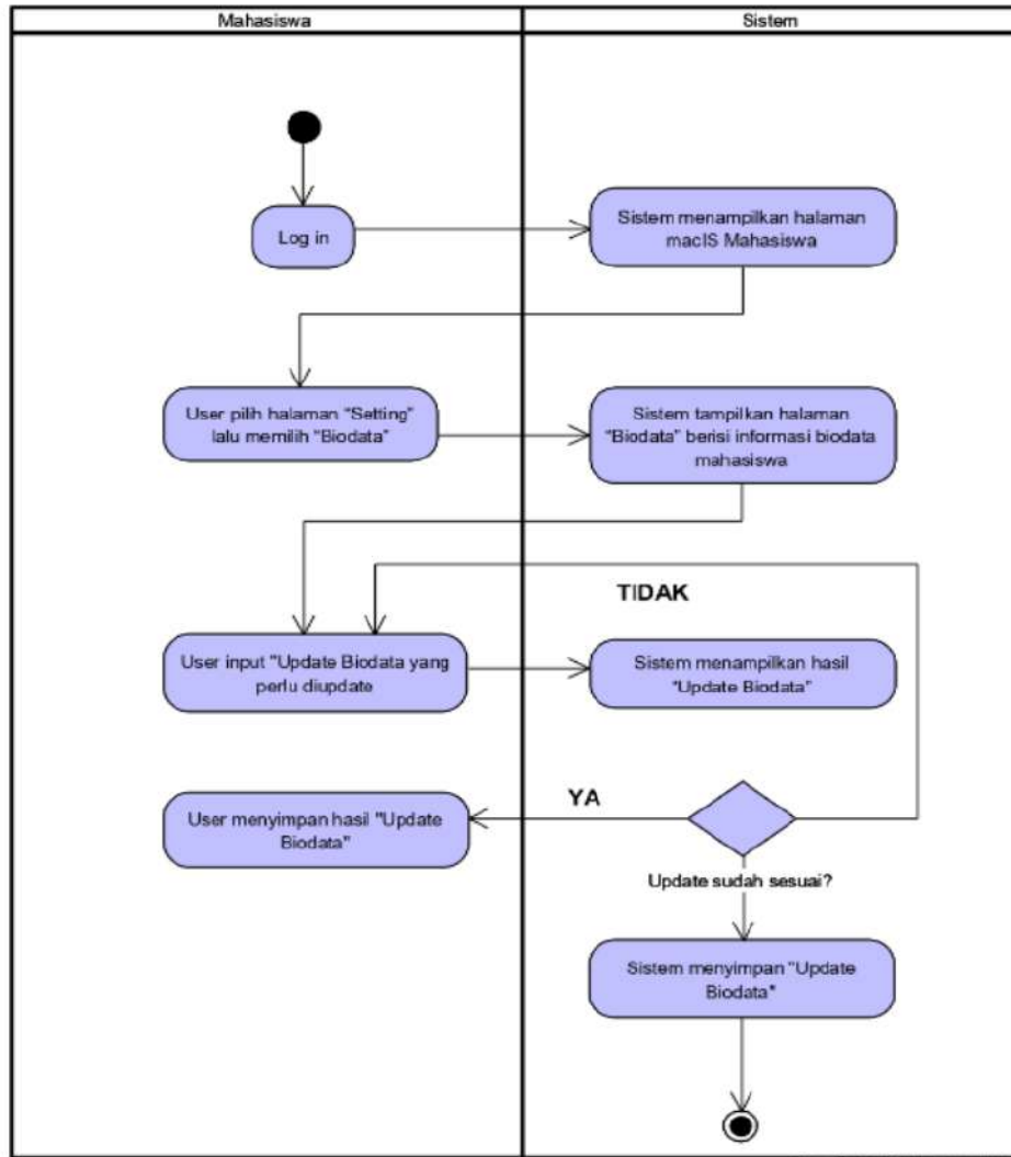
Gambar 9 Diagram Aktivitas Setting – Update Biodata
