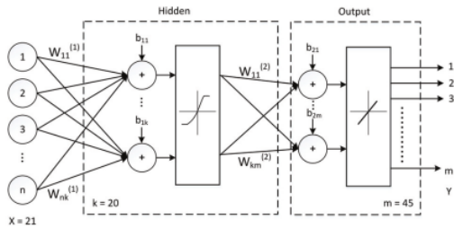
Fig. 8. Network type B: two-layer neural network with 45 output nodes.
