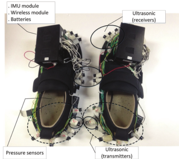
Fig. 1. The previous shoe-type measurement device.
