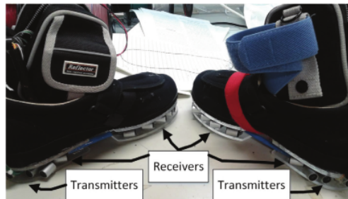
Fig. 3. The implementation of the position and angle of ultrasonic sensors based on the simulation.
