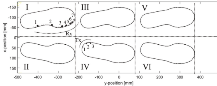
Fig. 2. The final representation of the region division, seven position of ultrasonic receivers (Rx), and three ultrasonic transmitters (Tx); were based on the previous study.
