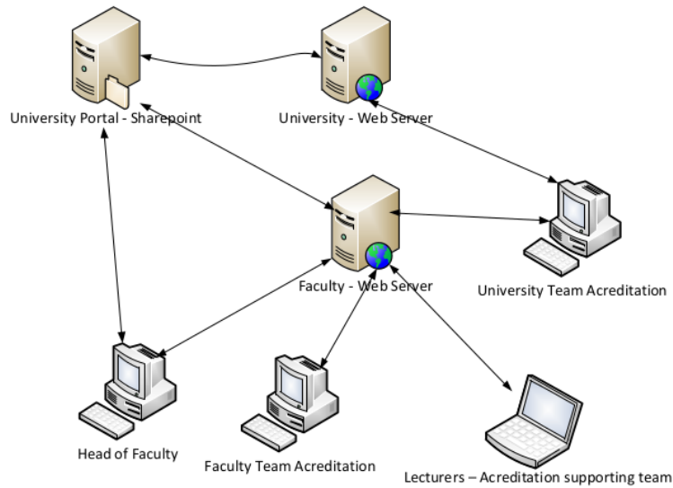
Figure 1. Architecture Diagram
