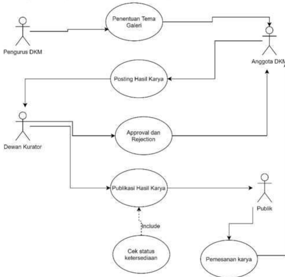
Gambar 2. Use Case Diagram Awal
