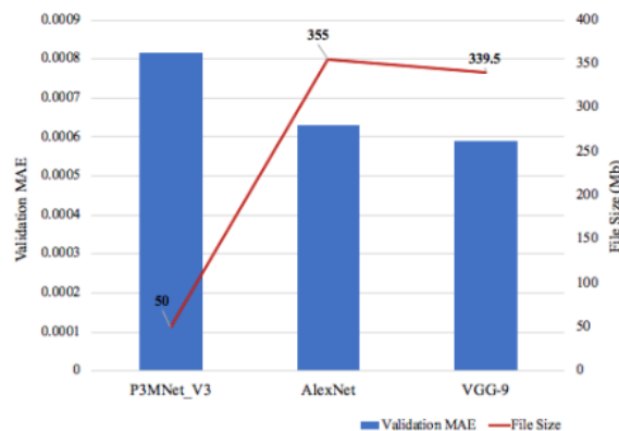
Figure 6. The MAE comparison of P3MNet_3, AlexNet and VGG-9 together with their trained models file size.
