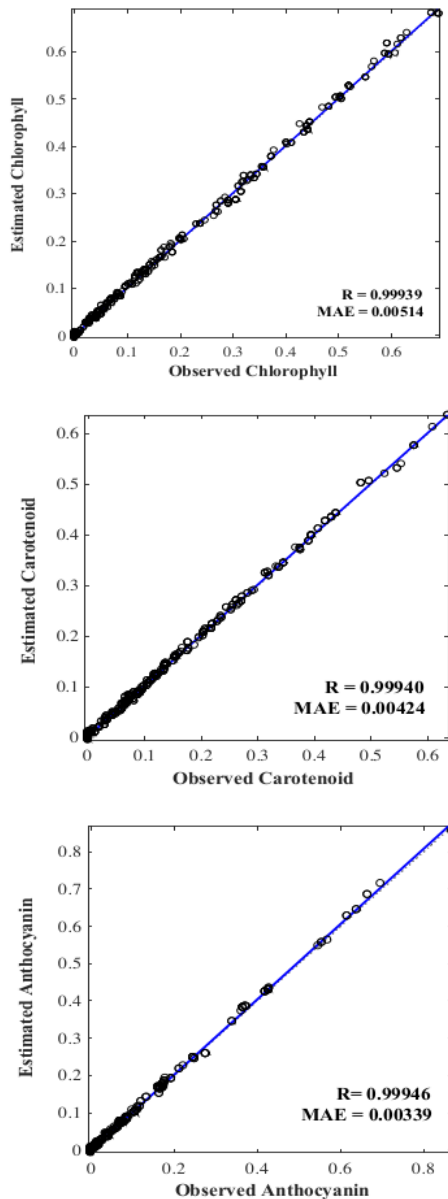
Figure 7. Performance of the P3MNet_3 for each pigment
