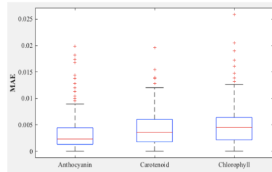
Figure 8. Boxplot of the validation MAE of P3MNet_3 for each pigment
