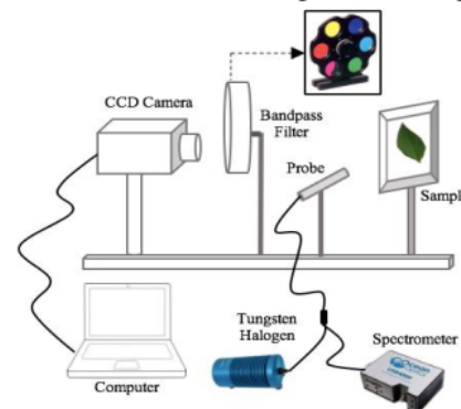
Figure 1. The devices arrangement for multispectral image acquisition
