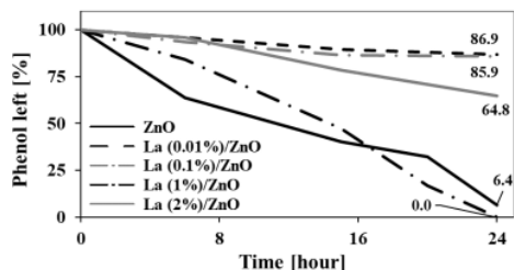
Figure 6. Photocatalytic phenol degradation on undoped ZnO and La-doped ZnO samples under UV light
