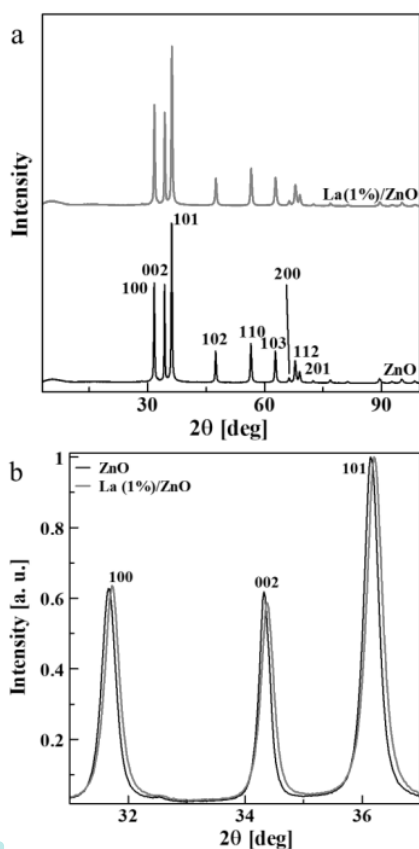
16 Figure 1. (a) XRD patterns of undoped and La(1%)/ZnO and (b) their respective magnification at selected diffraction planes
