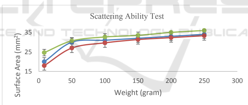
Figure 2: Scattering ability test diagram.
