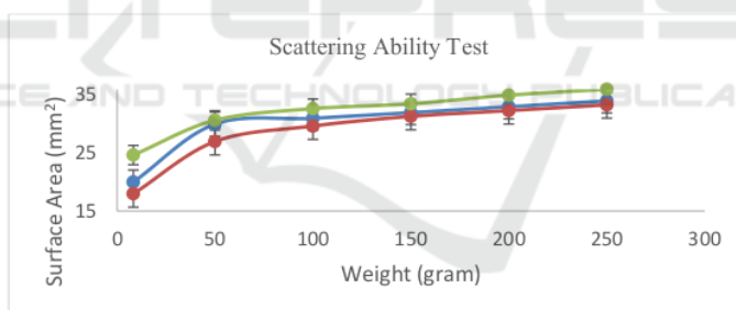
Figure 2: Scattering ability test diagram.
