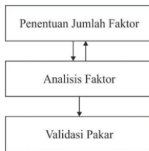
Gambar 2. Diagram analisis factor
