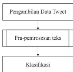
Gambar 1. Diagram analisis sentiment
