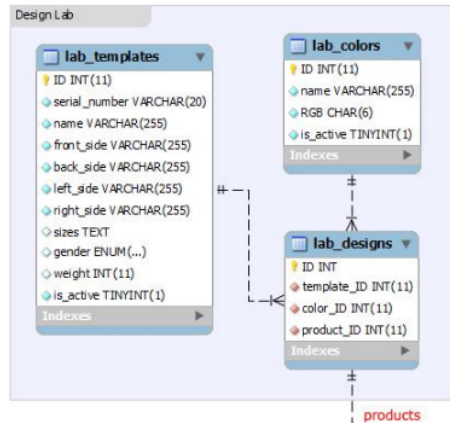
Gambar 7. Modul Design Lab
