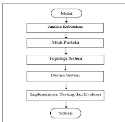
Gambar 8 Model Waterfall
