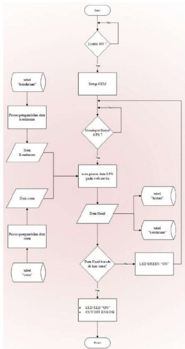
Gambar 10 Flowchart Prototipe
