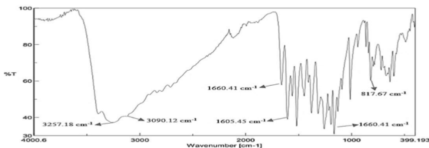
Figure 3: FT-IR spectrum of compound
