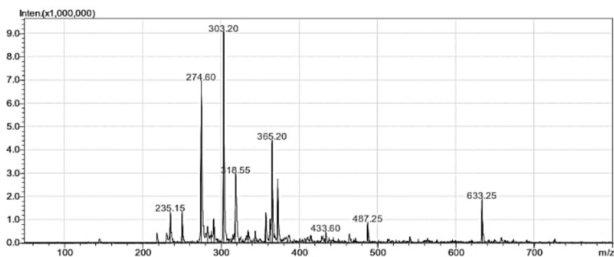
Figure 2: Mass spectrometry with Q1 scan mode (E+) of compound
