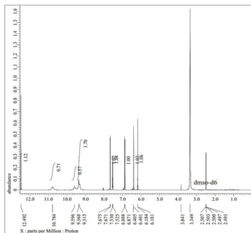
Figure 4: 1 H-NMR spectrum of compound ( \delta 0.000 – 12.000) (500 MHz)
