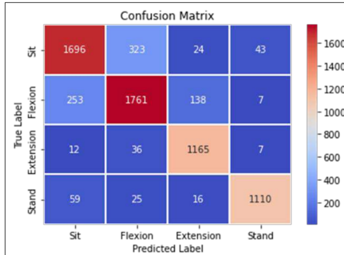
Figure 9 Confusion matrix of model classification results
