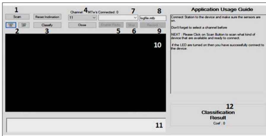
Figure 6 GUI application classifies STS movement in real time
