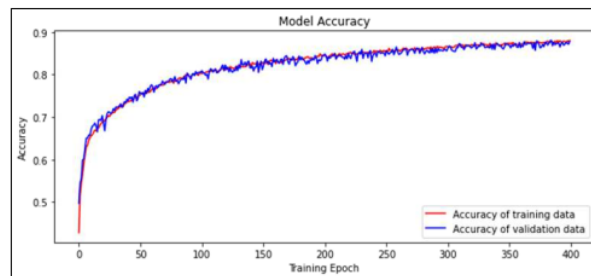
Figure 7 Graph Model of Accuracy
