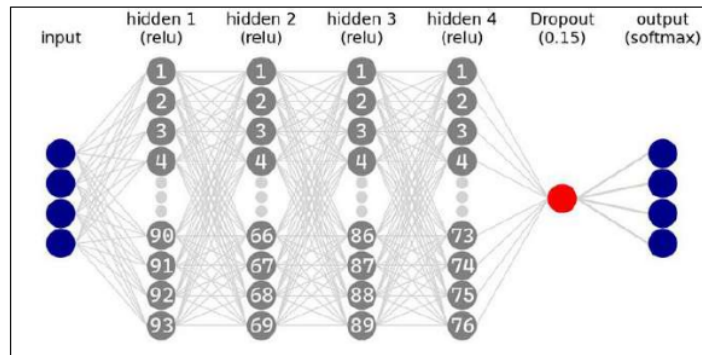
Figure 5 ANN architecture
