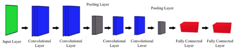
Figure 1. Architecture of MiniVGGNet.
