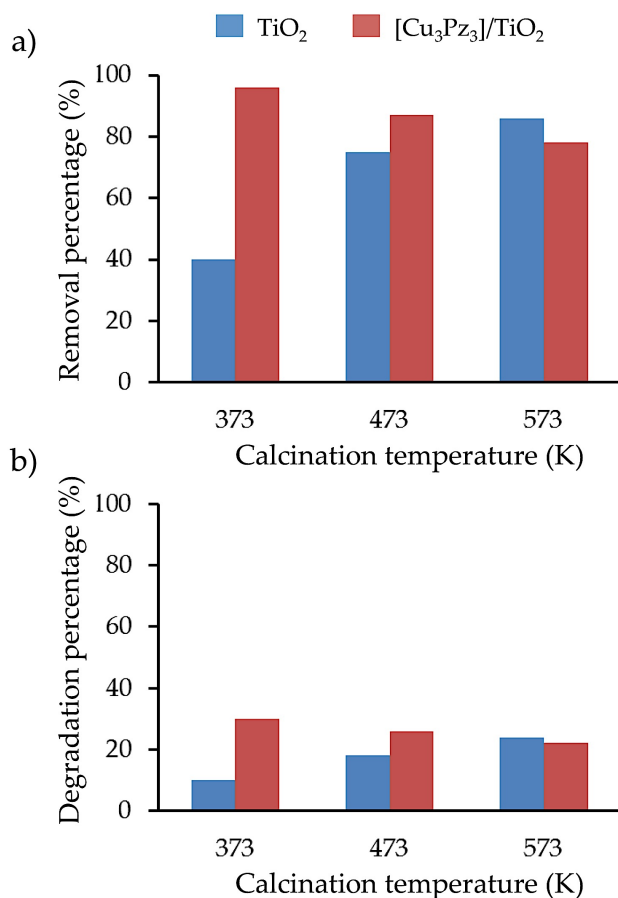
Figure 4. a) Removal and b) degradation percentage of TiO 2 and [Cu 3 Pz 3 ]/TiO 2 at different calcination temperatures.
