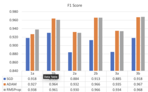
Figure 3. F1-Score graph.
