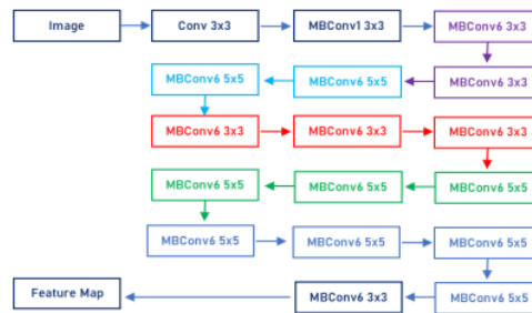
Figure 2. EfficientNetB0 architecture.
