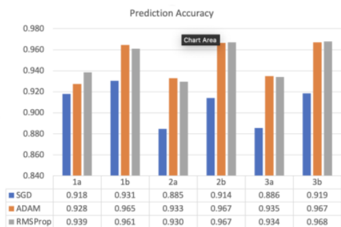
Figure 4. Prediction accuracy graph.
