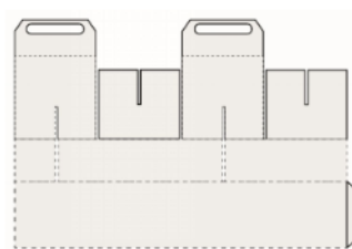
Gambar 14 Jari-jari kemasan family pack
