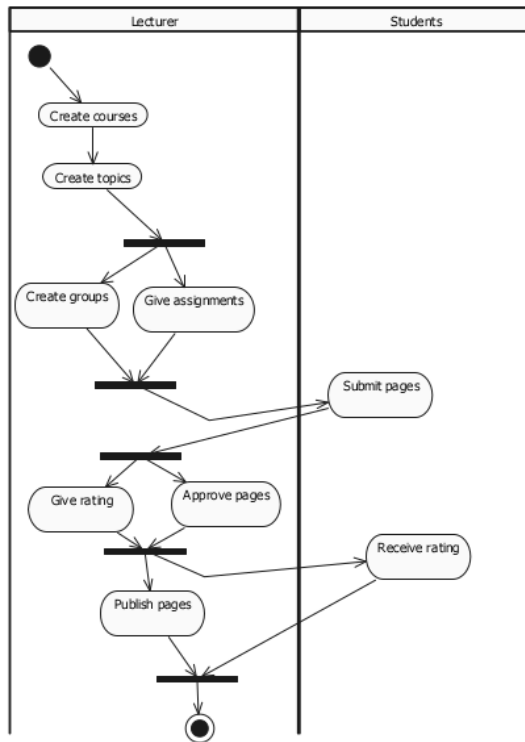
Figure 2. Activity Diagram
