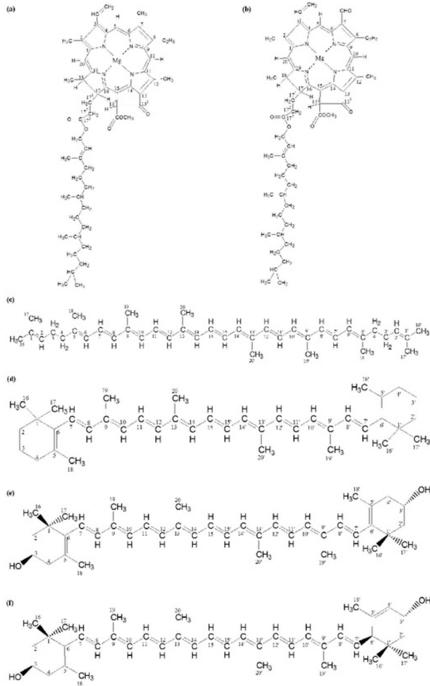
Figure 1. Chemical structure of Chl a (a), Chl b (b), lycopene (c), β-carotene (d), zeaxanthin (e) and lutein (f) with IUPAC numbering system.
