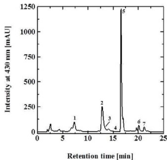
Figure 5. UFLC chromatogram of pigment extract from chloroplast of Pleomele angustifolia detected at 430 nm. The UFLC separation condition as follows: Pigment separation was performed using UFLC equipment with PDA (Shimadzu) on C30 column (150 × 4.6 mm I.D; YMC) with a gradient elution program of water, methanol and methyl tert-butyl ether (MTBE) at the flow rate of 1 mL/min at 30°C.
