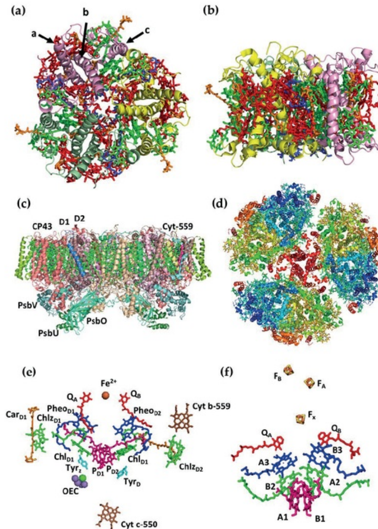
64 Figure 4. (a) A view looking down on the top of trimeric complex of LHCII structure from spinach. Each monomer is colored magenta, yellow and pale green. The three-transmembrane helices (a, b and c) present in a monomer are labeled and are easily visible. Chl a molecules are in red, Chl b colored green and carotenoids colored orange. (b) Side view of LHCII structure shows chlorophyll and carotenoid molecules are packed densely and close to each other (within van der Waals contact), enabling the crucial photoprotective role of these molecules to function by quenching triplet chlorophyll excited states. (c) Structure of PSII from Thermosynechococcus elongatus [28], a side-view representation of overall dimer perpendicular normal with the pseudo-twofold symmetry axis. (e) PSII core reaction center shown; component co-factors of the electron transport chain viewed along the membrane plane. The two branches are related by the pseudo-twofold symmetry axis. The respective pairs of pigments on the branches are labeled to indicate whether the Mg^{2+} is coordinated by D1, D2. (d) Structure of PSI from Synechococcus elongatus [29]; overview of the complete trimer looking along the membrane normal from the stromal side with each polypeptide of the trimer colored differently and chlorophyll molecules given in green. The two main proteins that comprise a monomer are PsaA (yellow) and PsaB (magenta). The electron transport chains are in the center of each monomer. (f) PSI core reaction center component co-factors of the electron transport chain are viewed along the membrane plane. The two branches are related by the pseudo-twofold symmetry axis. The representative pair of chlorophyll molecules on the branches are labeled A or B indicating whether the Mg^{2+} is coordinated by PsaA or PsaB. The iron-sulfur center of F_x involves residues from both PsaA and PsaB, while F_A and F_B are located in an extrinsic subunit called PsaC.
