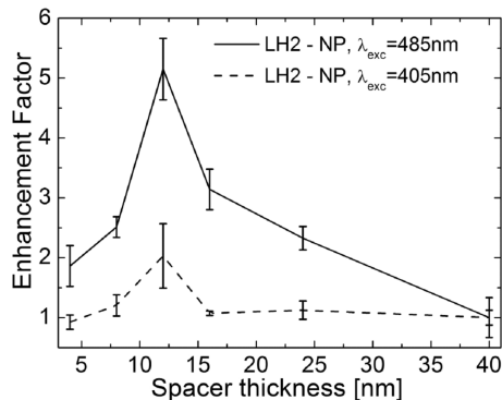
Fig. 3. Comparison of enhancement factor as a function of the spacer thickness for studied hybrid nanostructures. Solid line represents the on-resonance 485 nm excitation laser, while dashed line indicates the off-resonance 405 nm excitation laser.
