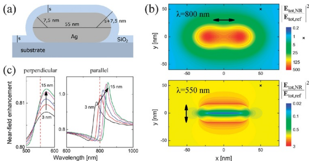
Fig. 5 (a) Schematic of the nanorod and the spacer structure considered for the calculations. (b) Maps of the electric field intensity enhancements |E_{\text{tot,NR}}/E_{\text{tot,ref}}|^2 calculated on the top of the spacer. The thickness of the spacer is set to s = 9 \text{ nm} . The wavelength of the incident light is set at, respectively, 800 nm and 550 nm for the light polarized parallel (upper map) and perpendicular (lower panel) to the symmetry axis of the nanorod. The polarizations are marked by the black arrows. (c) Spectra of the near field enhancement calculated for spacer thickness varying from 5 nm to 13 nm for the incident light polarized perpendicular (left panel) or parallel (right panel) to the long axis of the nanorod. Black arrows indicate the shifting of the resonance position with increasing spacer thickness. Spectra are calculated for points marked in (b) with black crosses. Red dashed lines indicate the wavelengths of interest – 550 nm and 800 nm.
