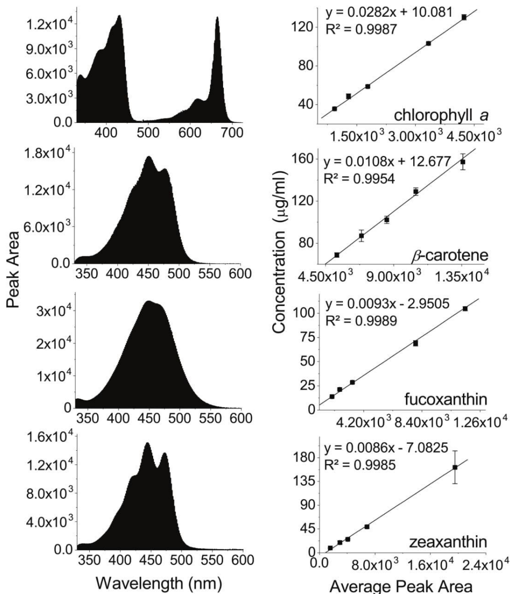
Figure 2. The histograms of the average peak area (left) and linear equation formula (right) of the standard pigments chlorophyll a, \beta -carotene, fucoxanthin, and zeaxanthin that were generated after multi-chromatogram calculation on the 3D HPLC data. Data were obtained from three repetitions and show average and SE.
