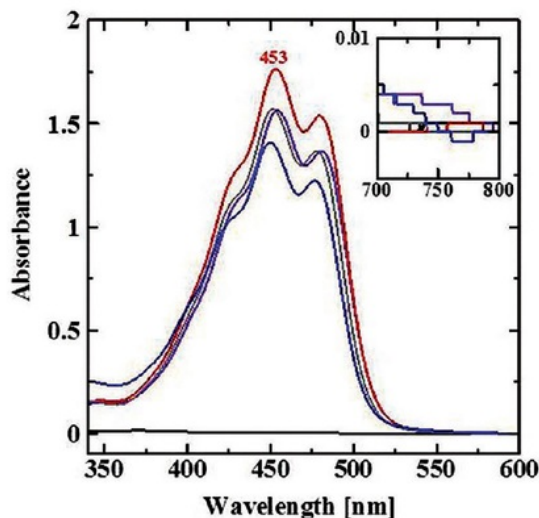
Figure 1. Absorption spectra of crude Car extracts from the cells of Erythrobacter sp. strain KJ5 extracted with 100% hexane (black), 100% acetone (violet), mixtures of MeOH and acetone (3:7, v/v) (red) and (7:3, v/v) (grey) and 100% MeOH (blue). Inset: absorption spectra of crude Car extracts in the range of 700–800 nm.
