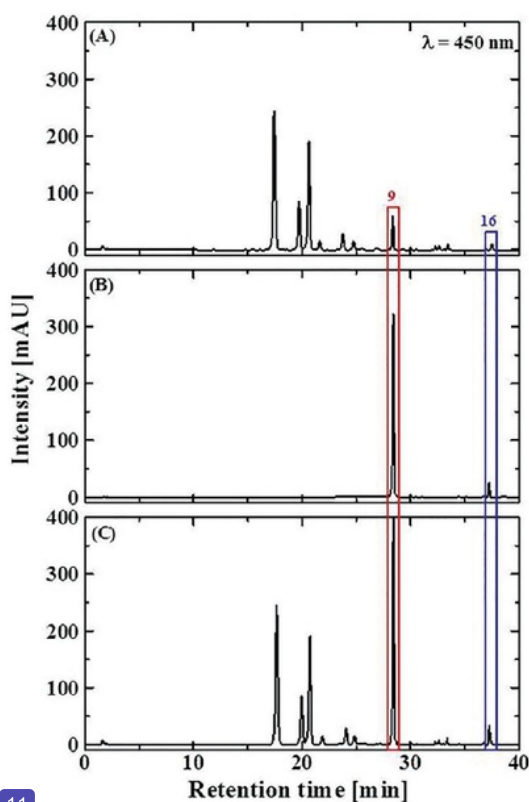
11 Figure 3. HPLC elution profiles of crude Car extract from the cells of Erythrobacter sp. strain KJ5 (A): a mixture of standards, zeaxanthin and \beta -carotene (B): Co-chromatography of crude Car extract with the standards, zeaxanthin and \beta -carotene (C). Peak 9 (red rectangle), zeaxanthin; and peak 16 (blue rectangle), \beta -carotene.
