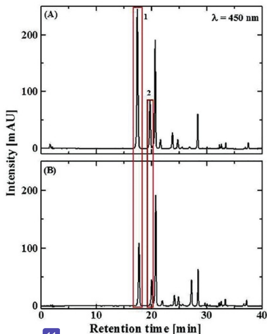
11 Figure 5. HPLC elution profiles of crude Car extract from the cells of Erythrobacter sp. strain KJ5 before (A) and after (B) saponification treatment. Note that after saponification (B), peaks 1 and 2 in red rectangles were obviously diminished.
