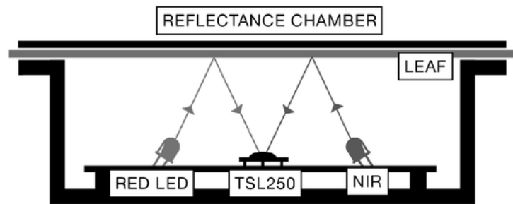
Figure 4. LCCM scanner reflectance mechanism chamber
