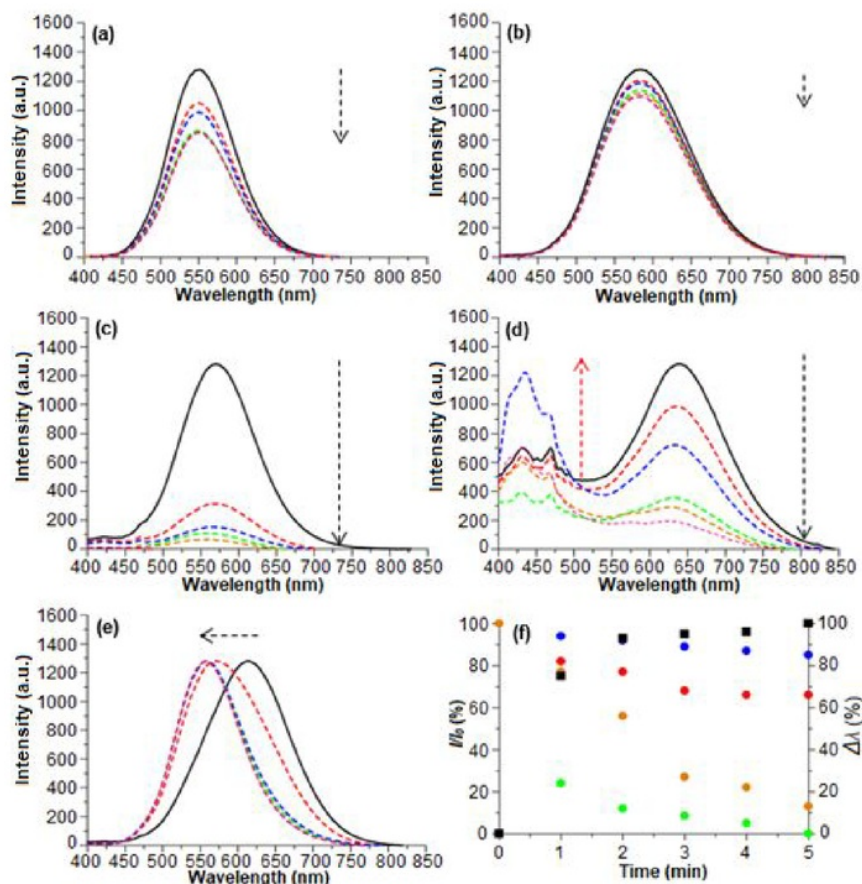
Fig 6. Emission spectral changes of (a) chemosensors 2_A ( \lambda_{\text{ext}} = 274 nm) (b) 2_B ( \lambda_{\text{ext}} = 280 nm) (c) 2_C ( \lambda_{\text{ext}} = 280 nm), (d) 2_D ( \lambda_{\text{ext}} = 322 nm) and (e) 2_E ( \lambda_{\text{ext}} = 278 nm) upon exposure to ethanol from 0 (black solid line), 1 (red dash line), 2 (blue dash line), 3 (green dash line), 4 (orange dash line) to 5 min (pink dash line) as well as (f) their changes in emission intensities for chemosensors 2_A (553 nm, red dot), 2_B (584 nm, blue dot), 2_C (570 nm, green dot), 2_D (644 nm, orange dot) and Stokes shift for chemosensor 2_E (616 nm, black square)
