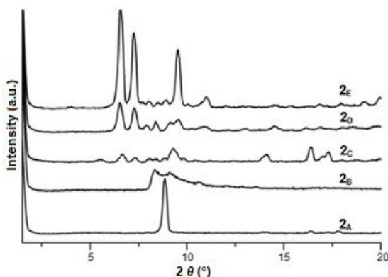
Fig 3. X-ray patterns of copper complexes 2 A-E
