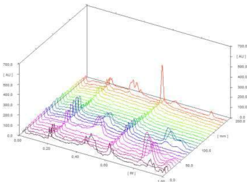
Figure 2. Densitogram at a wavelength of 200 nm
