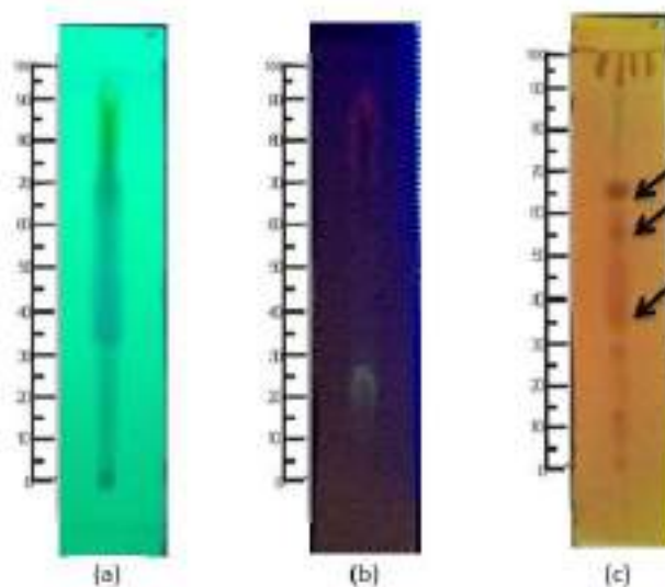
Figure 1. The result of (a) UV 254 Test, (b) UV 366 Test, and (c) Dragendorff Test on SQuR
