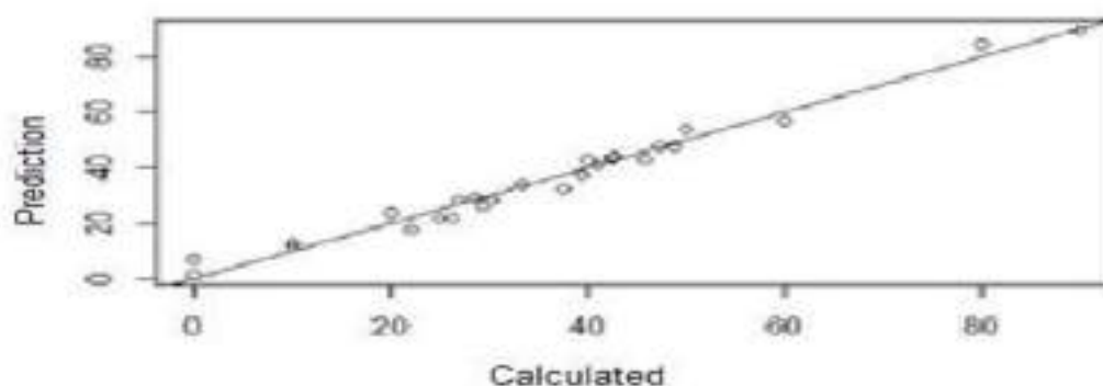
Fig. 3: Acetaminophen calibration curve
