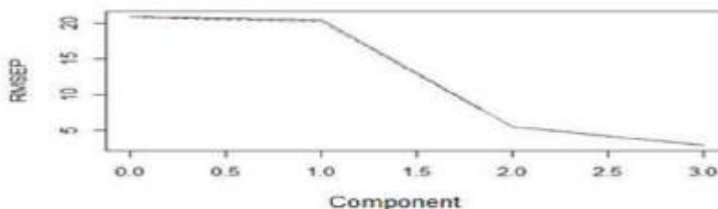
Fig. 2: RMSEP plot of acetaminophen
