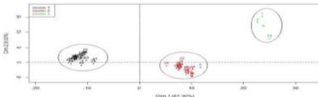
Fig. 7: Factor map diagram
