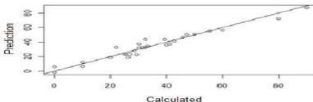
Fig. 5: Phenylbutazone calibration curve
