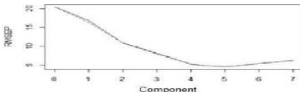
Fig. 4: RMSEP plot of phenylbutazone
